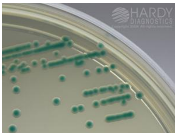
Cronobacter sakazakii (ATCC® 29004) colonies growing on HardyCHROM™ Sakazakii (Cat. no. G315). Incubated aerobically for 24 hours at 35 deg. C.
